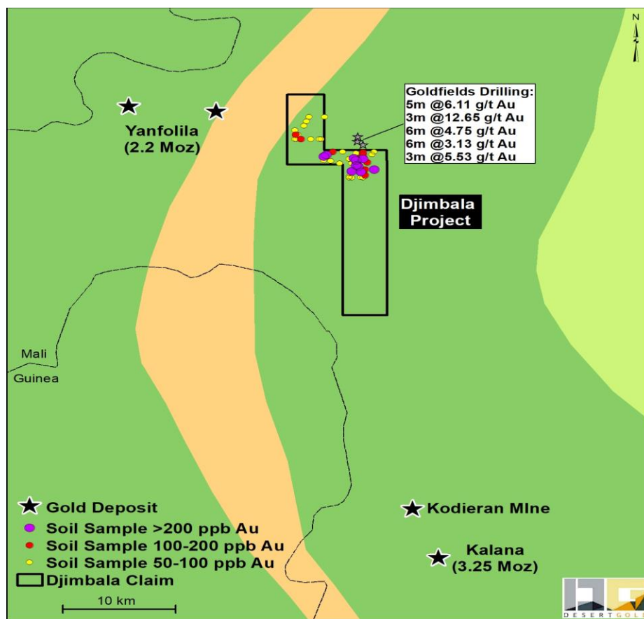
Figure 7: Location Plan of Djimbala Project
