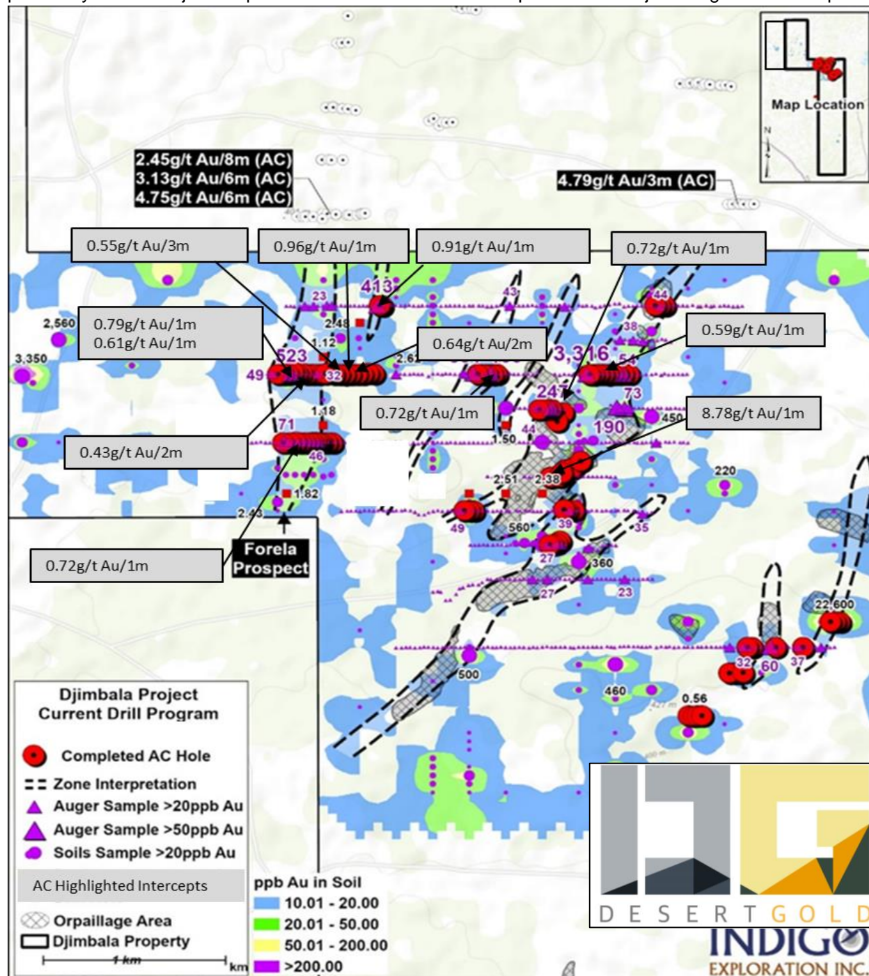
Figure 8: Forela, Djilefing and Nounssamna Gold Trends and Completed AC Drill Holes
